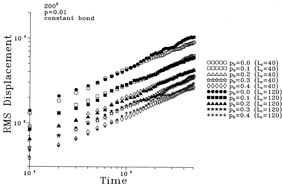
FIG. 4. Log-log plot of rms displacement (internal nodes) versus time of constant bond chains, for chain lengths L_c = 40 and 120 and barrier concentrations p_b = 0.0 - 0.4 . Same statistics as in Fig. 3.
